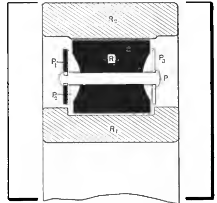
Fig. 2—Section through Norma roller bearing
